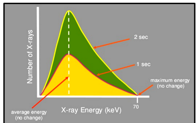
Fig. 5: Effect of exposure time on beam energy
