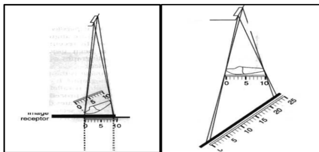
Fig. 15: Object-film alignment
