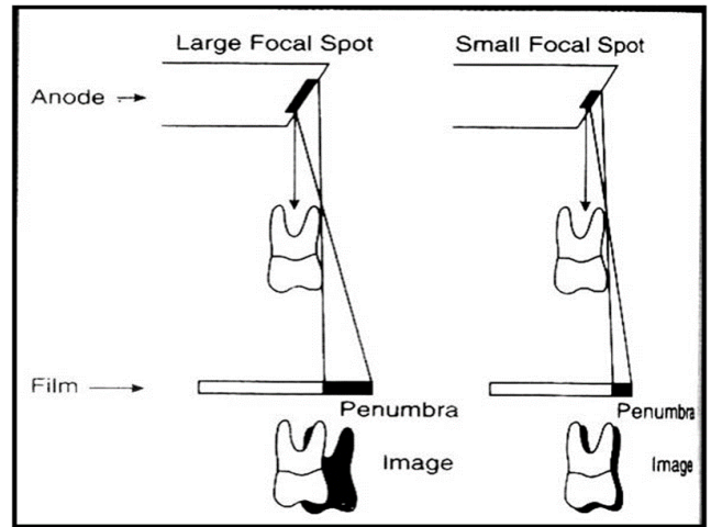
Fig. 10: Effect of focal spot size
