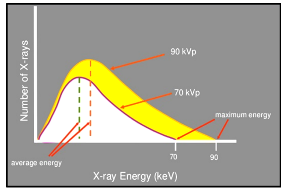
Fig. 3: Effect of tube voltage on beam energy
