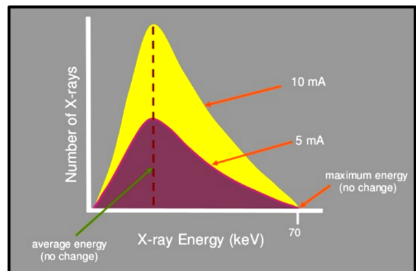
Fig. 4: Effect of tube current on beam energy
