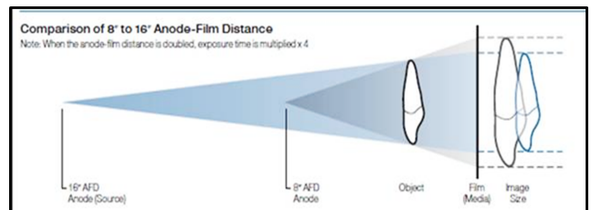
Fig. 11: Effect of target-film-distance
